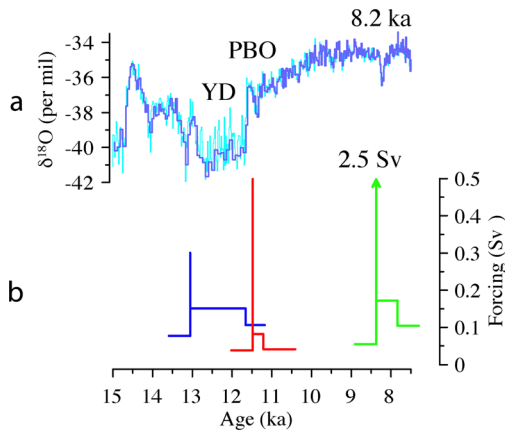
Figure 1. (a) The Greenland ice core (GISP2) \delta^{18}\text{O} record [Grootes et al. , 1993; Stuiver and Grootes, 2000]. (b) Freshwater fluxes used in our experiments, with initial 1-yr flood followed by increased flux associated with routing. Blue: fluxes used for Younger Dryas (YD) simulation [Licciardi et al. , 1999; Leverington et al. , 2000]. Red: fluxes used for Preboreal Oscillation (PBO) simulation [Licciardi et al. , 1999; Fisher et al. , 2002]. Green: fluxes used for the 8.2-ka event simulation [Licciardi et al. , 1999; Clarke et al. , 2004].
