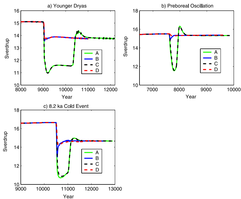
Figure 2. Time series of maximum meridional overturning (in Sverdrup) for model simulations of (a) the Younger Dryas, (b) the Preboreal Oscillation and (c) the 8.2-ka event. Please refer to Tables 1 to 3 for a description of model simulations A to D for each meltwater event.
